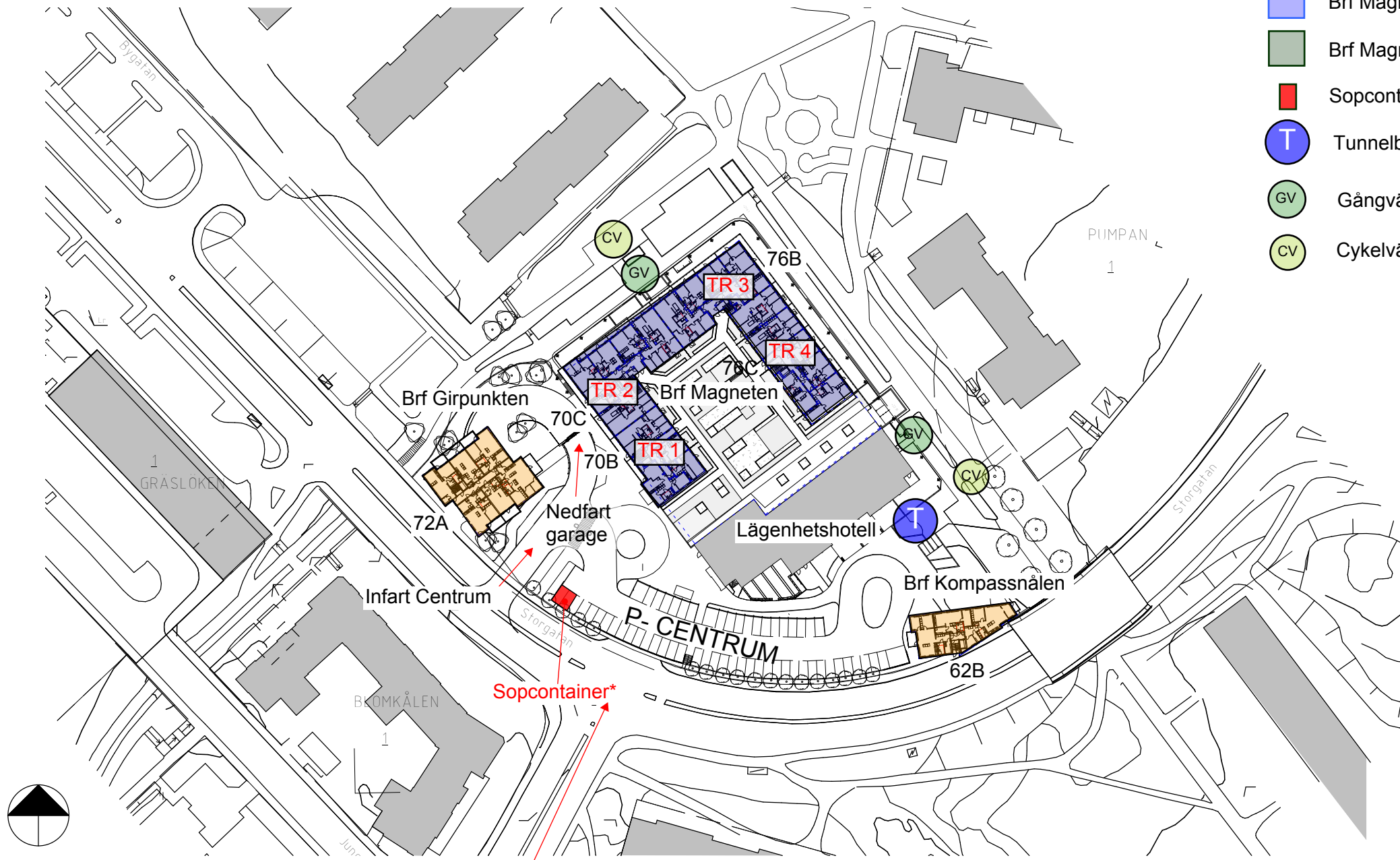
BRF MAGNETEN, SITUATIONSPLAN
